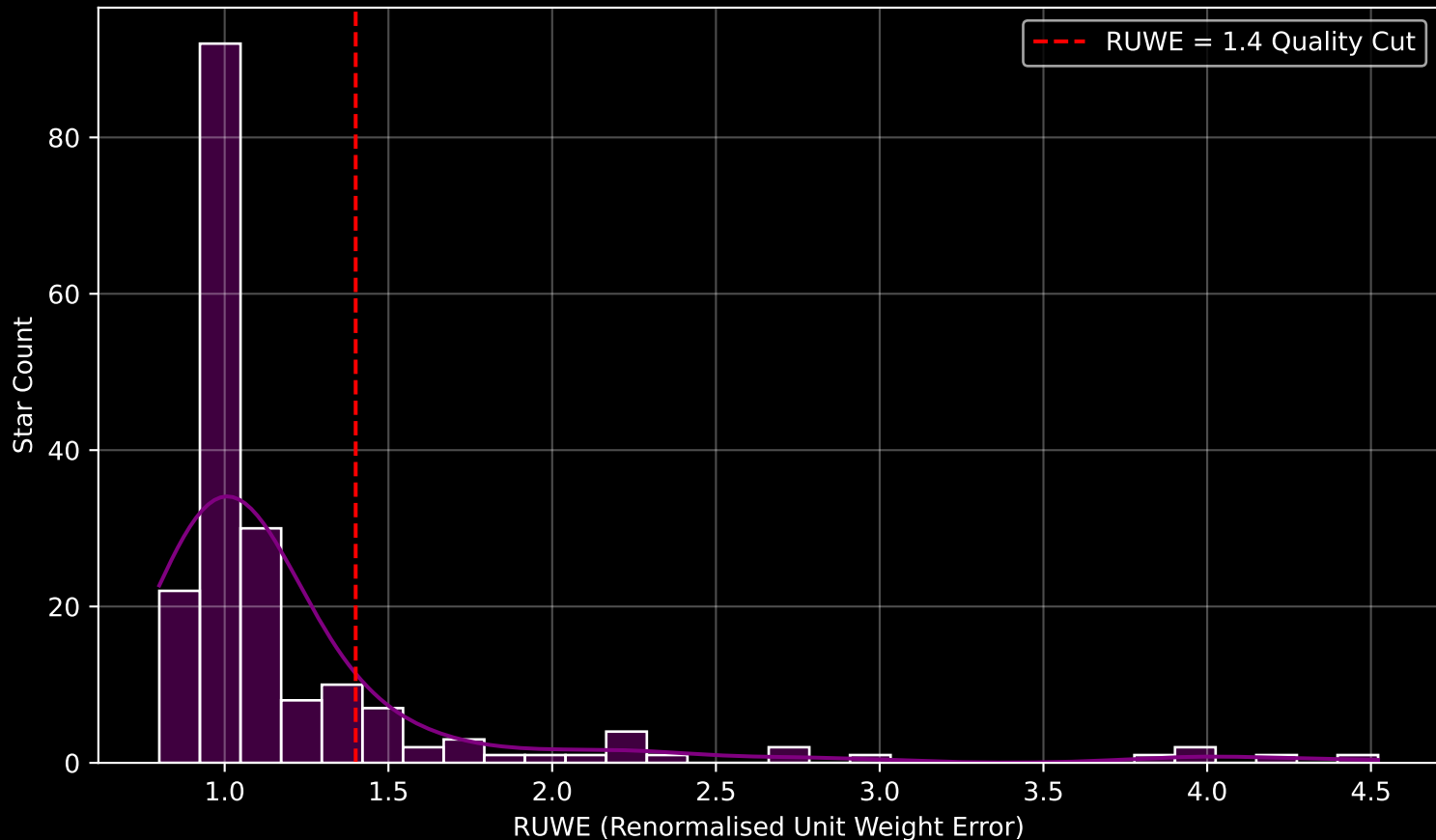
GAPOGEE DR17 Field [105-30] RUWE Distribution (n= 190)
