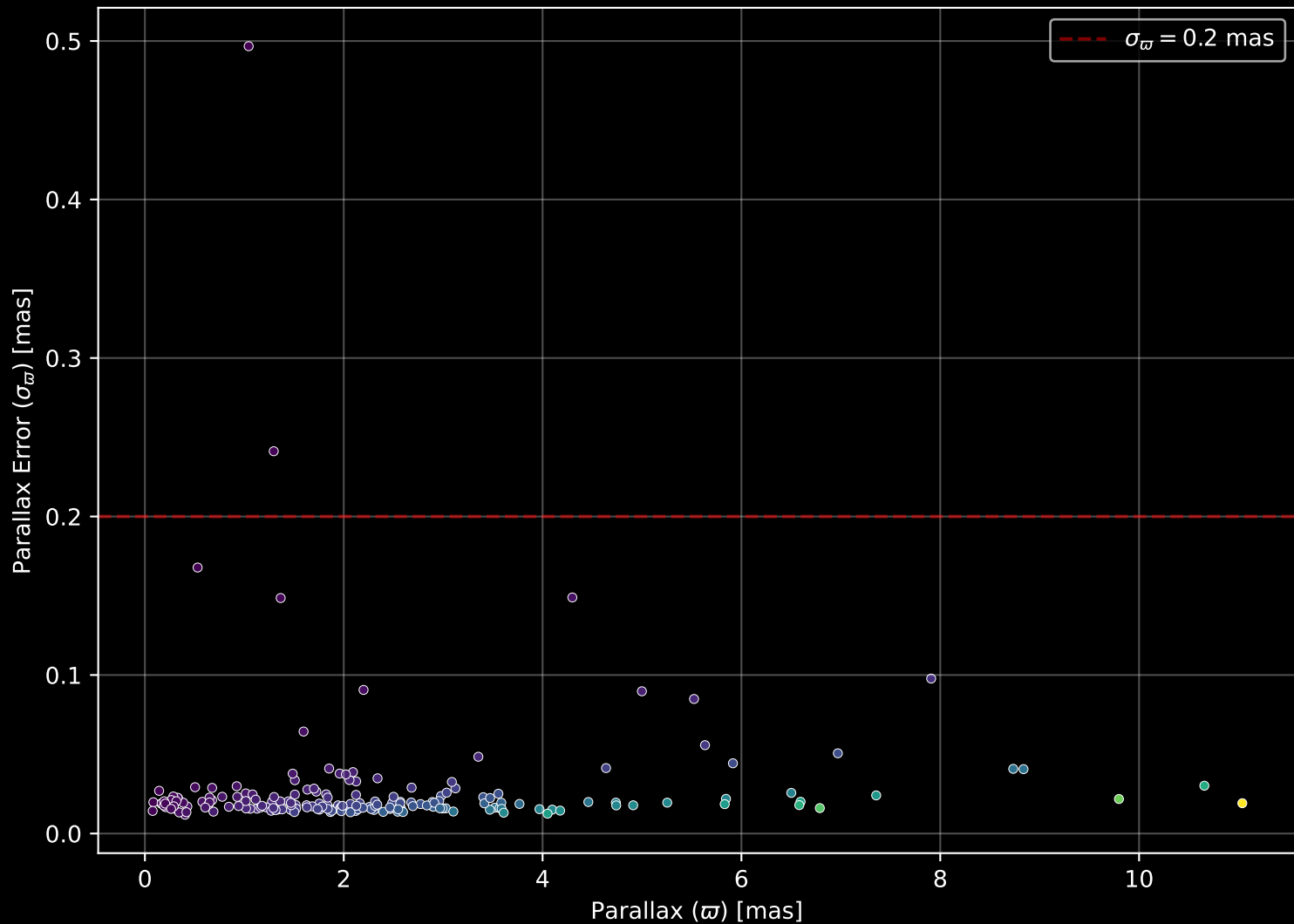
APOGEE DR17 Field: [105-30] Parallax Quality (n= 195)
