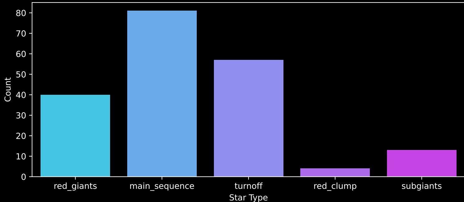
APOGEE DR17 Field: [105-30] Count plot of Star Type
