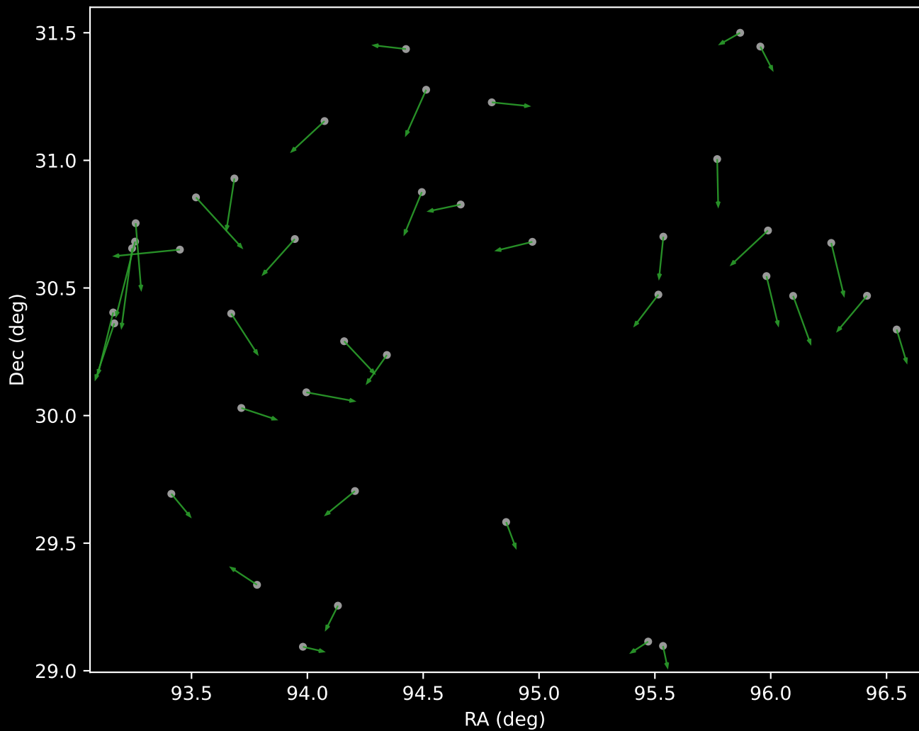
APOGEE DR17 Cluster 4 Proper Motion Vectors (n=40)
