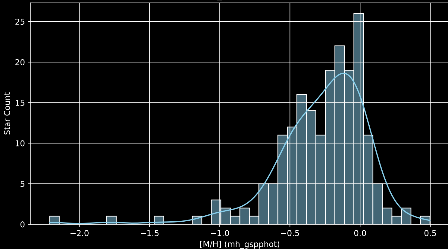
APOGEE DR17 Field: [105-30 [M/H] (mh_gspphot) (n= 195)
