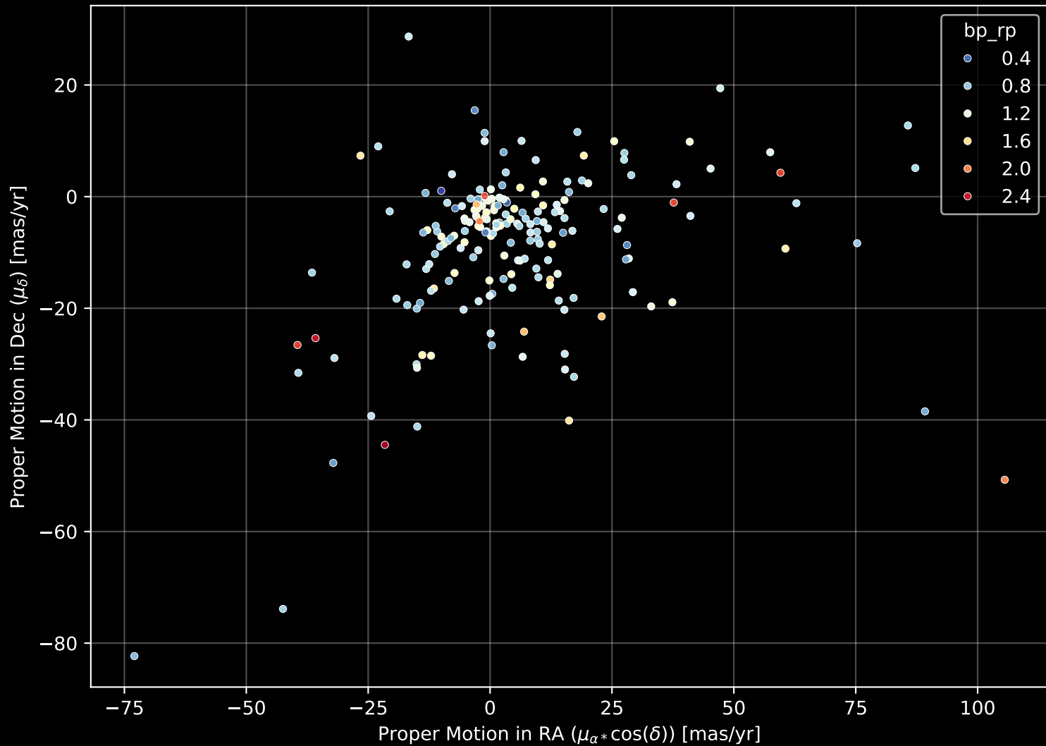
APOGEE DR17 Field: [105-30] Proper Motion Diagram (n= 195)
