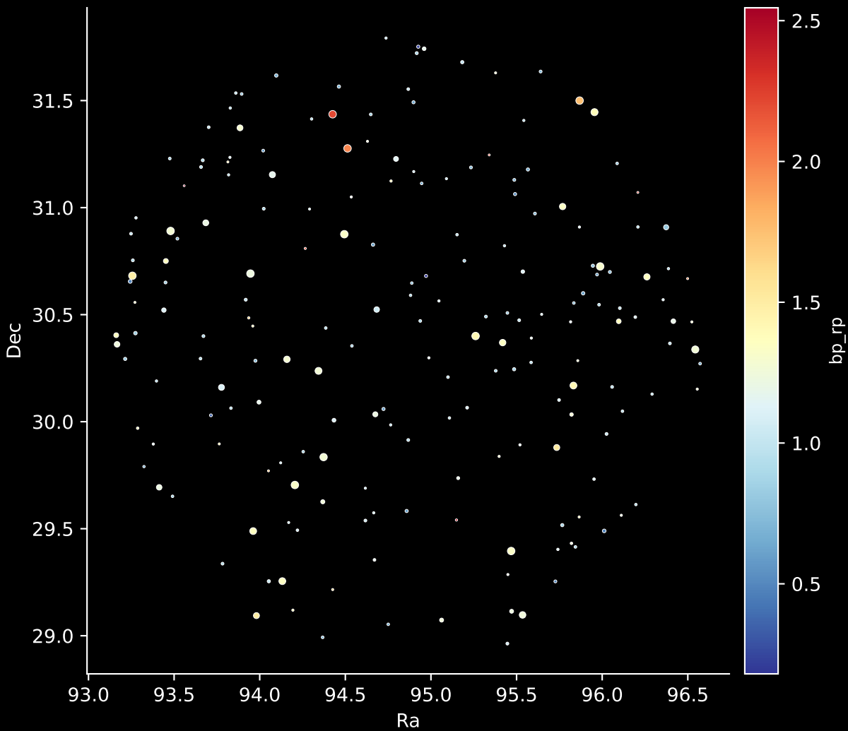
APOGEE DR17 Field: [105-30] Stars: 195
